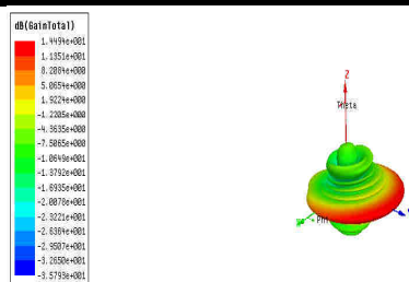
Fig.10: Typical 3-D Radiation pattern of Non Inclined Narrow wall slotted waveguide array with Irises.
